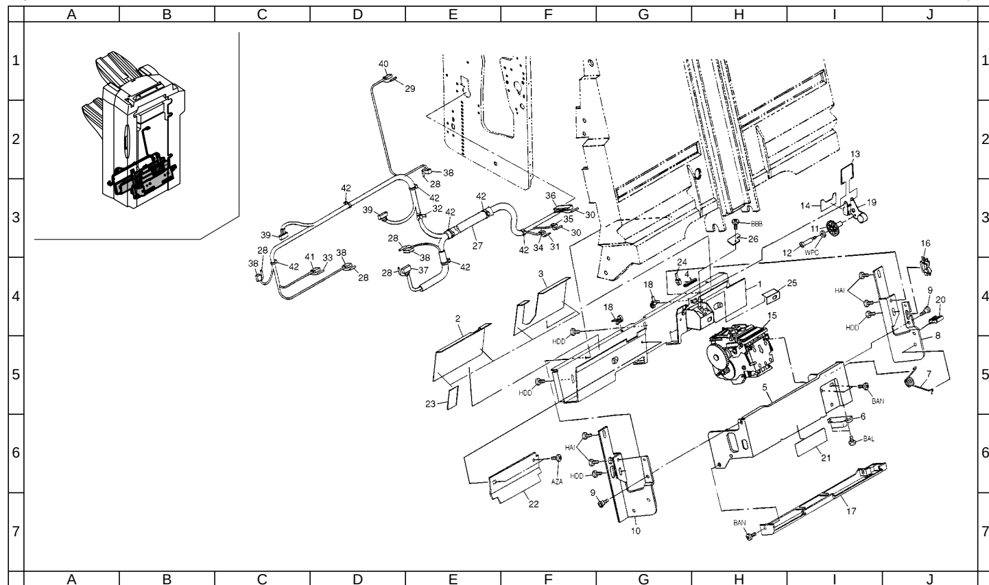
FIG. 7 MIDDLE TRAY 2
