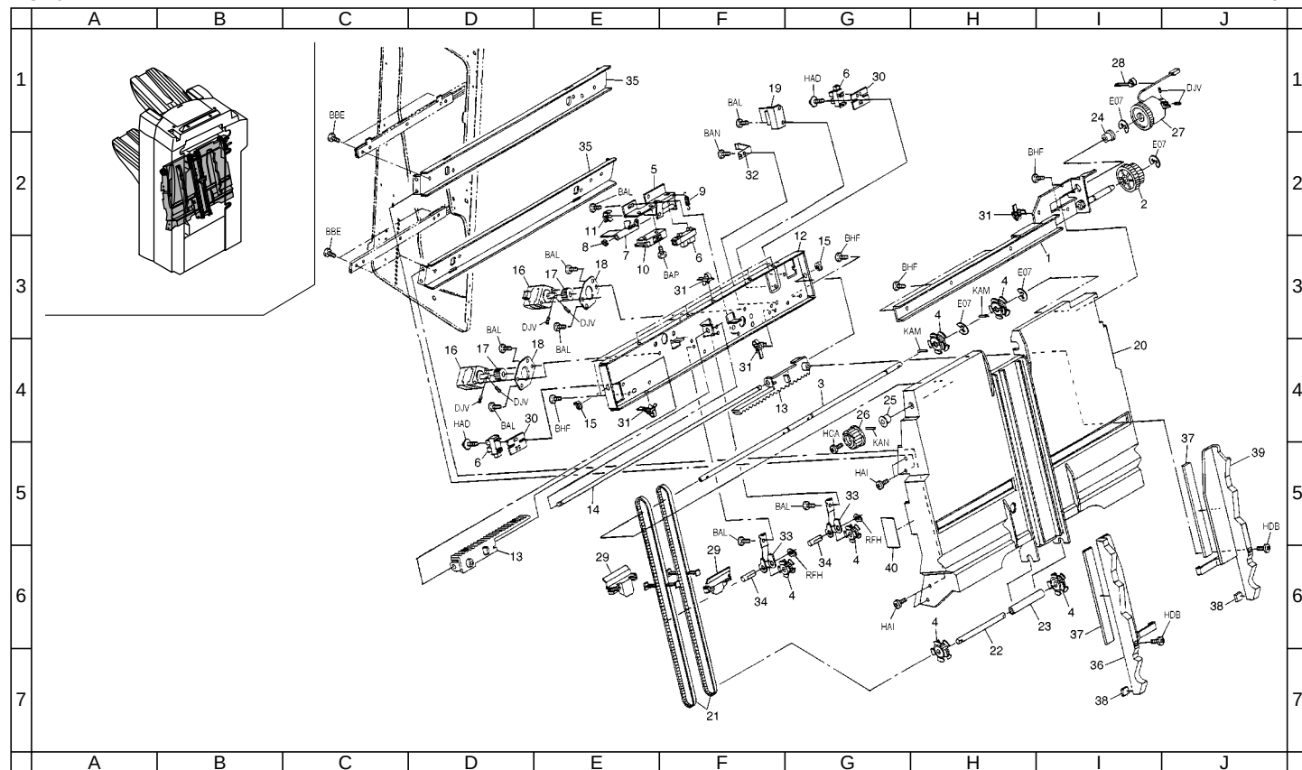
FIG. 6 MIDDLE TRAY 1
