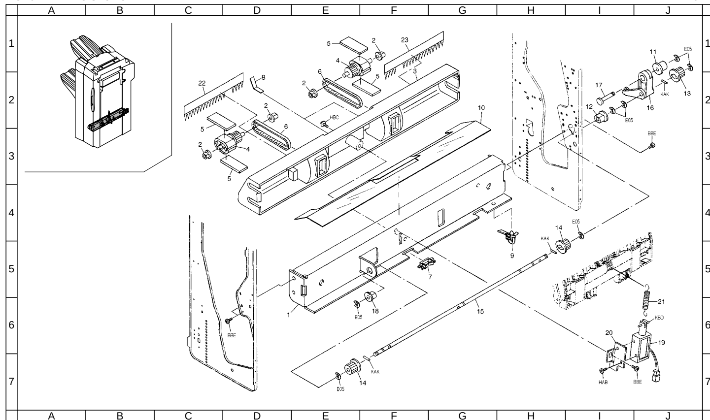
FIG. 9 DRIVING SECTION 2
