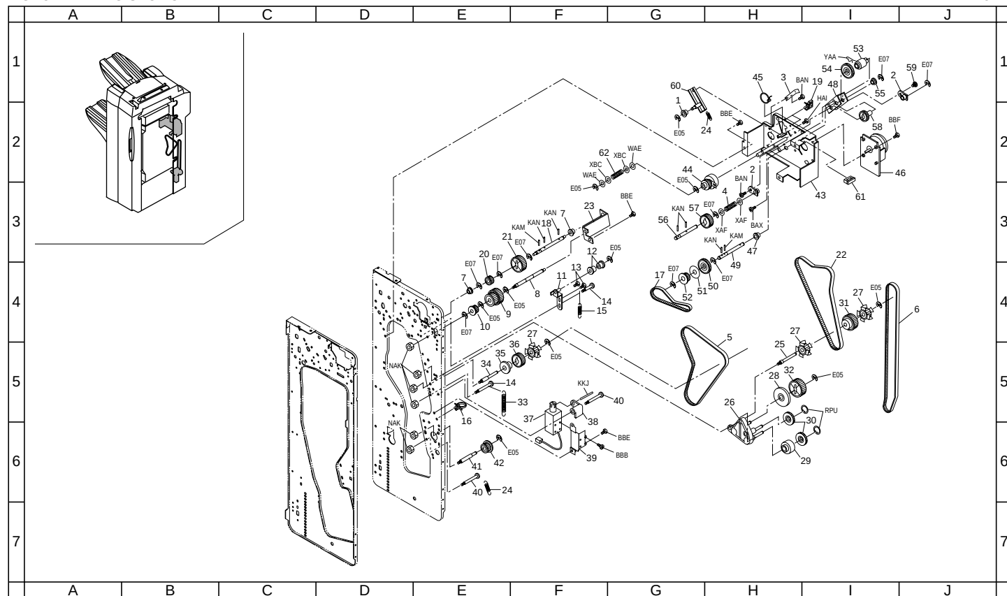
FIG. 8 DRIVING SECTION 1
