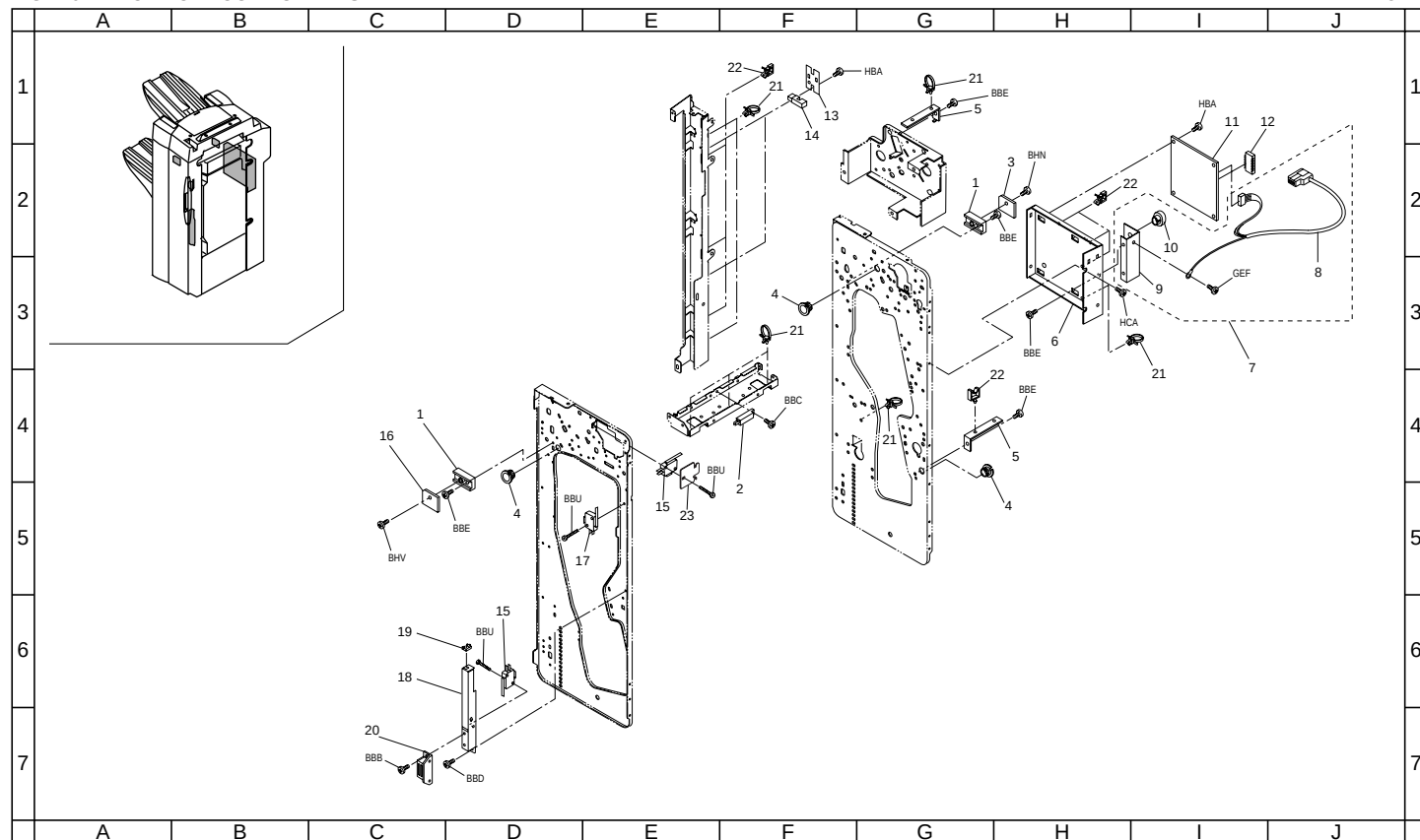
FIG. 10 ELECTRICAL COMPONENTS 1
